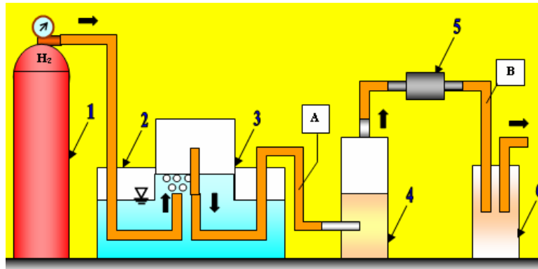
1 – pressure vessel, 2 – outer container, 3 – measuring cylinder, 4 – container with silica gel, 5 – filter, 6 – drain container \text{SiO}_2
