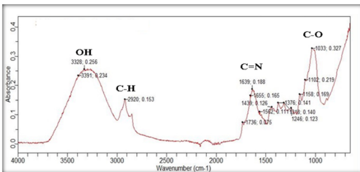
FIGURE 4: FTIR image for modified plantain peel.
