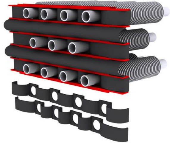
FIGURE 8: Rubber seals on the inlet side of the exchanger
