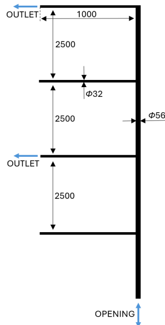
FIGURE 2: Location of individual collection points in a four-story apartment building
