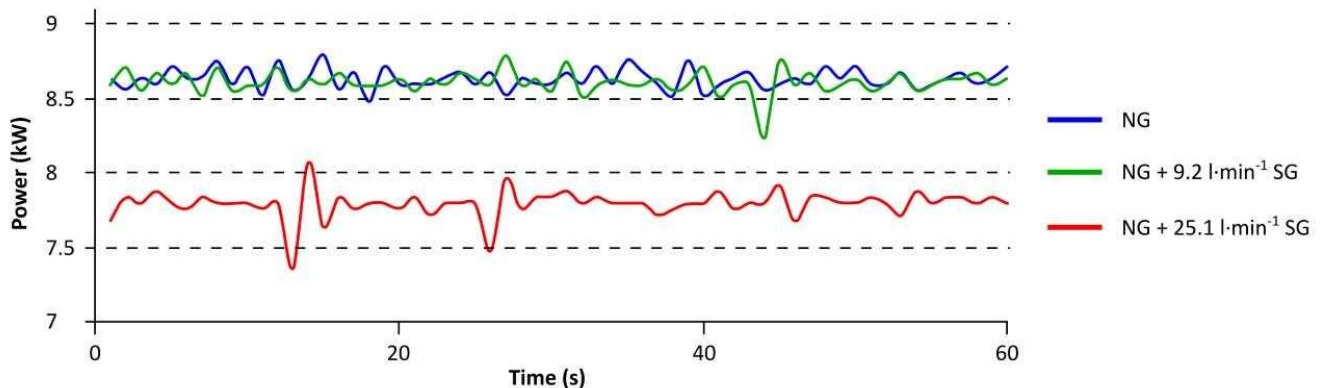
FIGURE 2: Power of the electric generator depending on the composition of the fuel mixture
