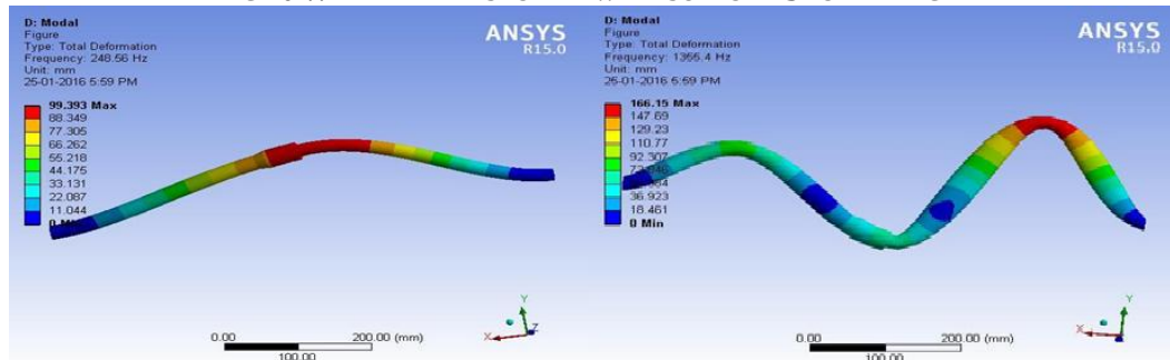
FIG 10 WITH MR ELASTOMER WITH SUPPORT SHORT LENGTH
