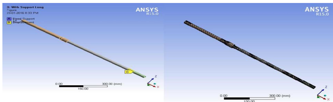
FIG 5 THE ELECTRIC TRIMMER HAS FOLLOWING CONSTRAINED ON ROD
