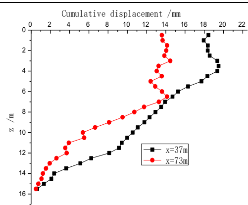
FIG. 7 CUMULATIVE HORIZONTAL DISPLACEMENT CURVE OF THE SOUTH SIDE OF FOUNDATION PIT
