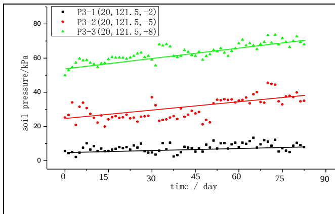
FIG. 8 EARTH PRESSURE CHANGE CURVE ( x=20M)
