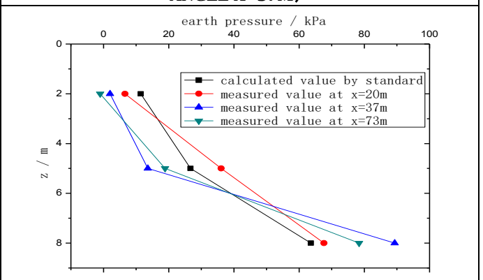
FIG. 11 COMPARISON VALUE OF EARTH PRESSURE BETWEEN MEASURED AND CALCULATED VALUE BY STANDARD
