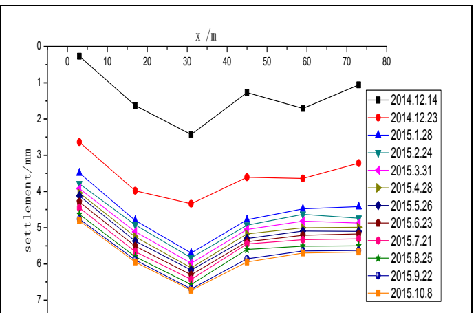
FIG. 3 SETTLEMENT CURVE OF THE SOUTH SIDE OF FOUNDATION PIT
