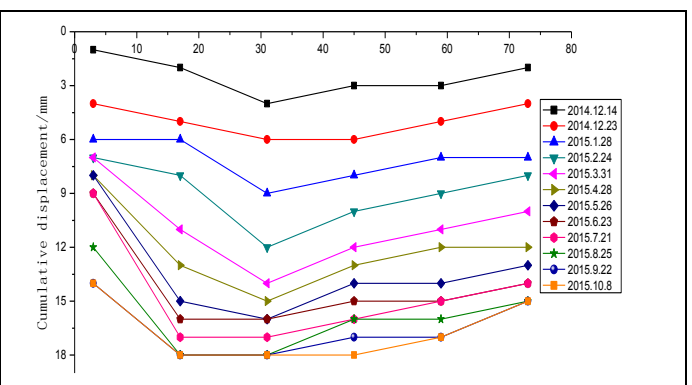
FIG. 5 HORIZONTAL DISPLACEMENT CURVE OF THE SOUTH SIDE OF FOUNDATION PIT
