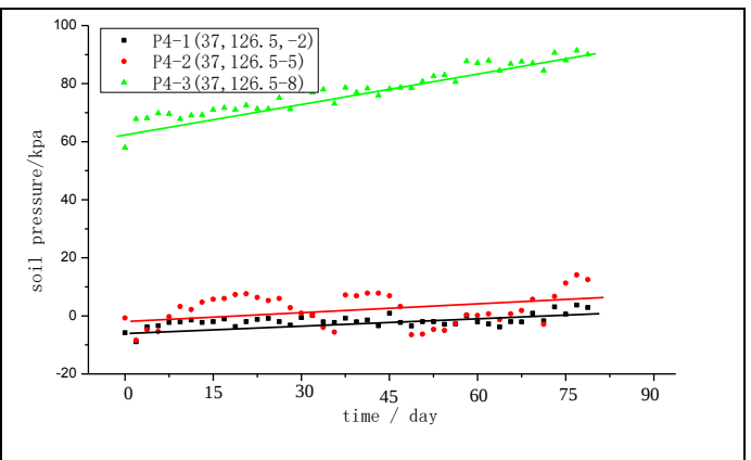
FIG. 9 EARTH PRESSURE CHANGE CURVE ( EXTERNAL ANGLE X=37M)
