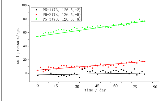
FIG.10 EARTH PRESSURE CHANGE CURVE ( NEGATIVE CORNER X=73M)
