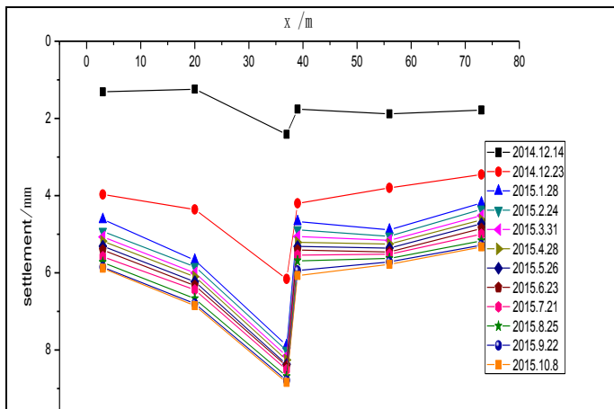
FIG. 2 SETTLEMENT CURVE OF THE NORTH SIDE OF FOUNDATION PIT
