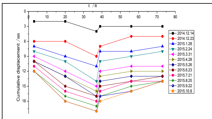
FIG. 4 HORIZONTAL DISPLACEMENT CURVE OF THE NORTH SIDE OF FOUNDATION PIT
