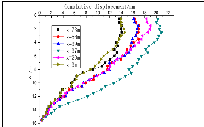
FIG. 6 CUMULATIVE HORIZONTAL DISPLACEMENT CURVE OF THE NORTH SIDE OF FOUNDATION PIT
