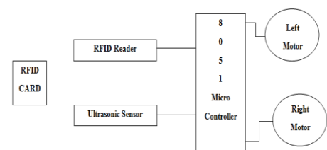
FIG.6. BLOCK DIAGRAM OF ROBOT NAVIGATION
