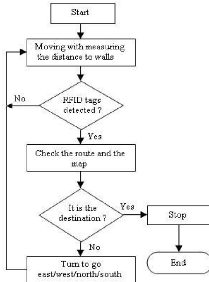
FIG.7. FLOW CHART SHOWING FUNCTIONING OF KIT
