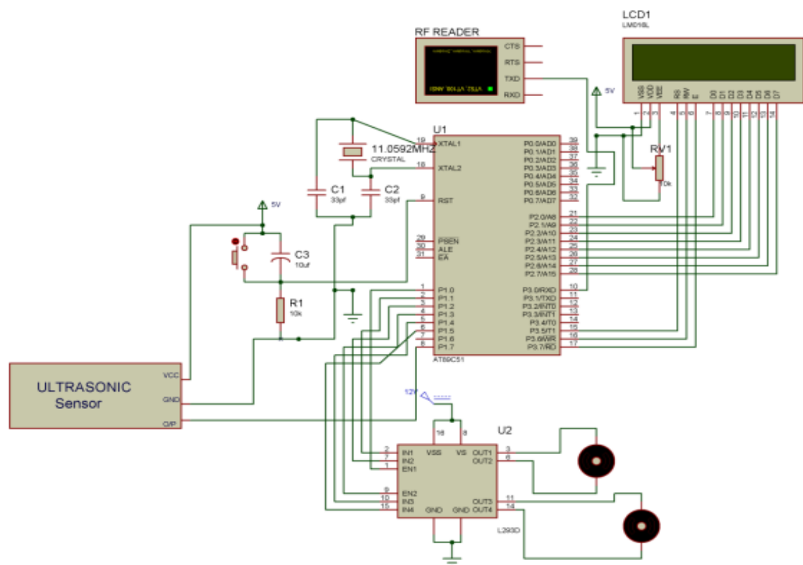
FIG.3 HARDWARE IMPLEMENTATION SCHEMATIC DIAGRAM
