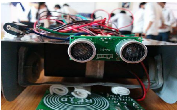
FIG.8.FRONT VIEW OF ULTRASONIC SENSORS
