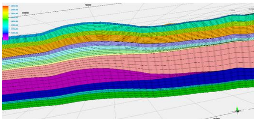
FIGURE 7: THE LAYERING IN THE MISHRIF FORMATION
