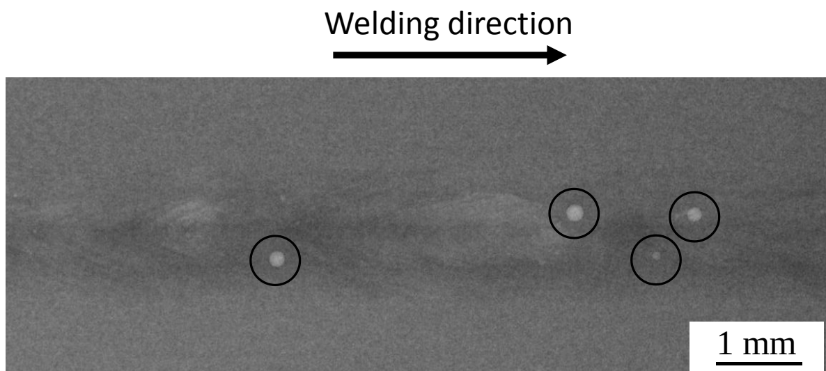
FIGURE 3: X-ray radiographic observation showing microporosities in the fusion zone of a weld ( P = 2230 \text{ W} , V = 3.7 \text{ m/min} , \text{Øf} = 153 \mu\text{m} )
