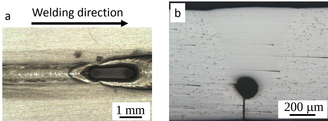
FIGURE 2: Optical observations with defects in the welds: (a) face view of molten pool collapse ( P = 2000 \text{ W} , V = 2.75 \text{ m/min} , \text{Øf} = 305 \mu\text{m} ), (b) Cross section evidencing lack of penetration and associated root porosity ( P = 2500 \text{ W} , V = 4.5 \text{ m/min} , \text{Øf} = 600 \mu\text{m} )
