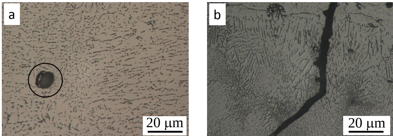
FIGURE 4: Optical micrographs showing (a) porosity ( P = 2000 \text{ W} , V = 2.27 \text{ m/min} , \phi_f = 134 \mu\text{m} ) and (b) cracking in the fusion zone of a weld ( P = 2500 \text{ W} , V = 2.5 \text{ m/min} , \phi_f = 675 \mu\text{m} )
