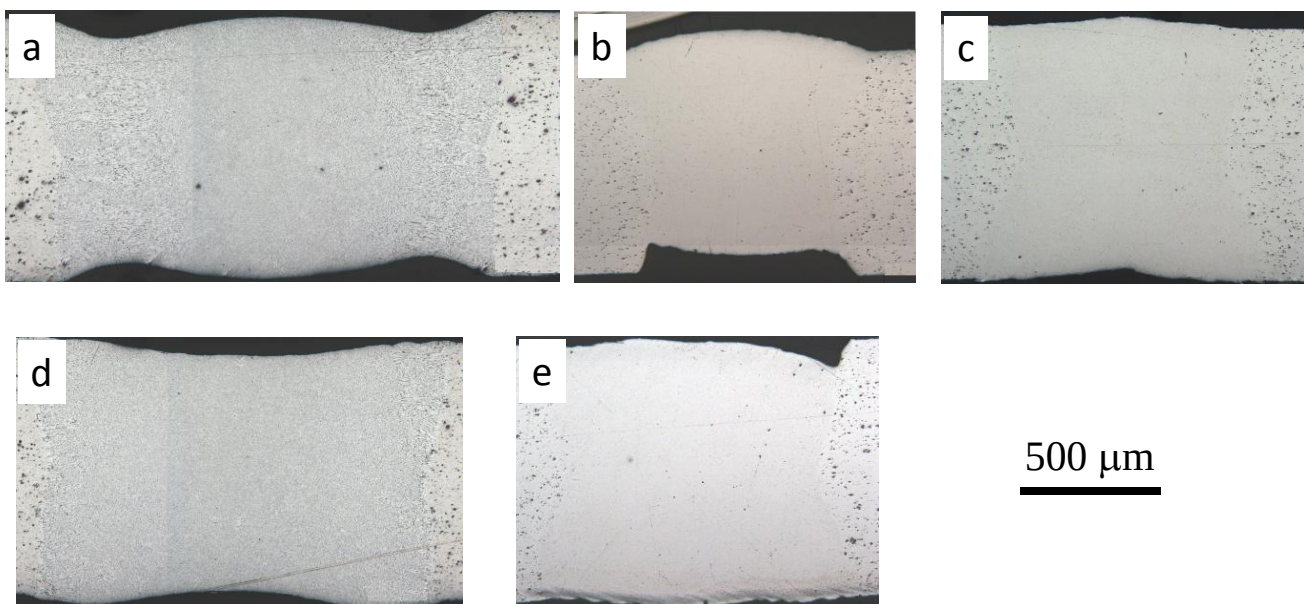
FIGURE 5: Non-conforming weld bead micrographs: (a) P = 900 \text{ W} , V = 7.05 \text{ m/min} , \phi_f = 195 \mu\text{m} , (b) P = 2500 \text{ W} , V = 8 \text{ m/min} , \phi_f = 370 \mu\text{m} , (c) P = 1000 \text{ W} , V = 2.75 \text{ m/min} , \phi_f = 240 \mu\text{m} (d) 1000 \text{ W} , V = 6.25 \text{ m/min} , \phi_f = 175 \mu\text{m} , (e) P = 2000 \text{ W} , V = 8 \text{ m/min} , \phi_f = 305 \mu\text{m} .
