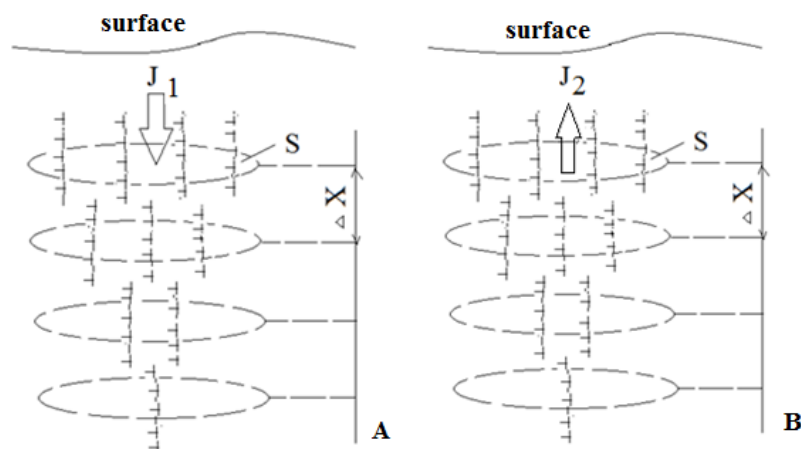
FIGURE 3: Scheme showing a qualitative change in the direction of the flow gradient of the dislocation density with increasing and decreasing changes in the value of stresses inside the nickel crystal lattice with increasing distance or depth from the surface: A-increase in the value of internal stresses; B-decrease in the value of internal stresses.
