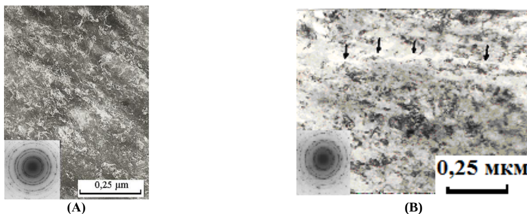
FIGURE 2: Formation of nanostructures at t = 0.9 \text{ ks} on the nickel surface at nominal contact pressure: a) 84 kPa; b) 168 kPa
