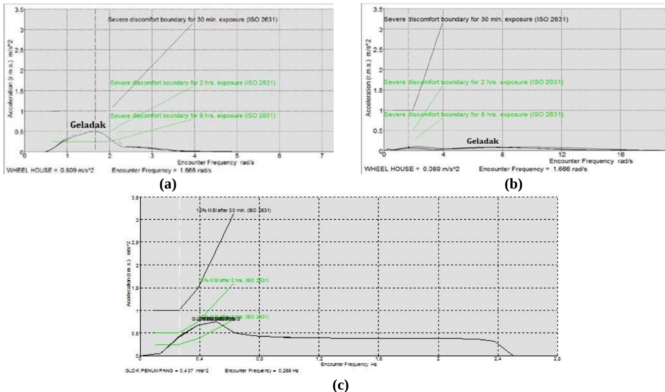
FIGURE 8: MSI ships Trimaran S/L = 0.2, (a) Heading Seas ( 180^\circ ), (b) Following Seas ( 0^\circ ), (c) Quartering Seas ( 45^\circ )
