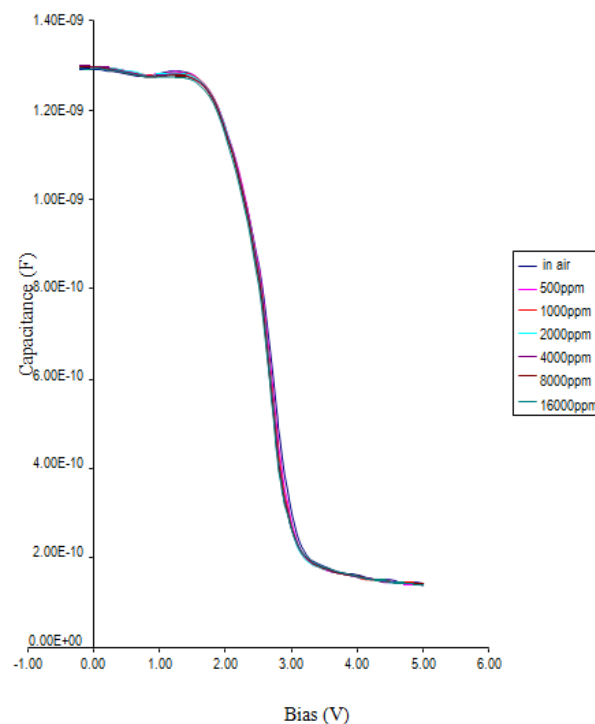
FIGURE 5: C-V response of Pd gate MOS sensor at 120°C
