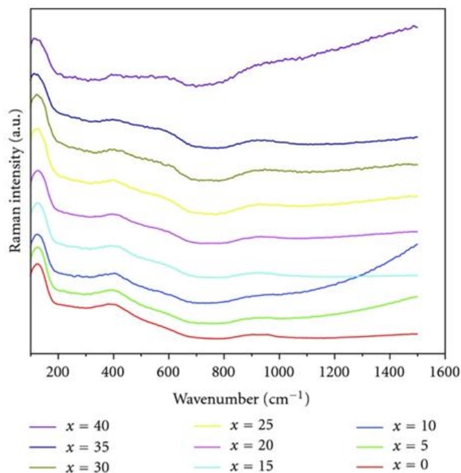
FIGURE 4: Raman spectra at room temperature for various 40\text{SiO}_2 \cdot x\text{ZnO} \cdot (60 - x)\text{Bi}_2\text{O}_3 crystal compositions.[27]
