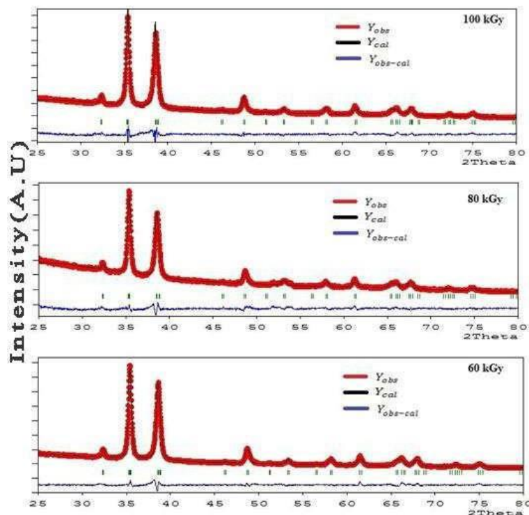
FIGURE 1: Refined output graph for different intensities (60 KGy, 80 KGy, 100 KGy)
