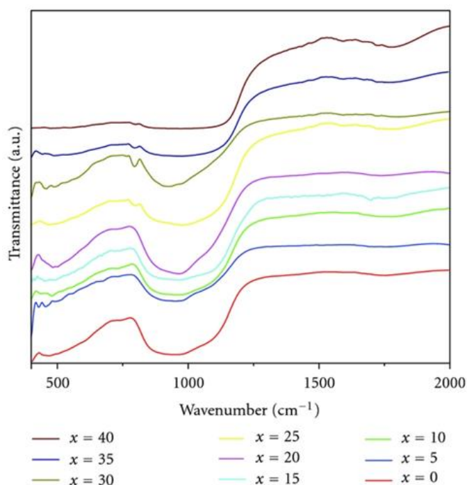
FIGURE 5: Infrared spectrum for various compositions of 40\text{SiO}_2 \cdot x\text{ZnO} \cdot (60 - x)\text{Bi}_2\text{O}_3 at room temperature.[27]
