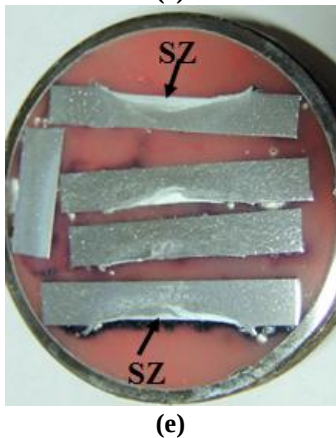
FIGURE 1: (a) The Al-Sc equilibrium phase diagram, (b) Schematic diagram of double-pass FSPed set-up (plate size: 150 \times 90 \times 8 \text{ mm}^3 ), (c) Tool configuration, (d) Double-pass FSPed plate (each impression contain double-pass FSP), (e) A bunch of macrostructures of double-pass FSPed as showing of stir zone (SZ), (f) A bunch of tensile test samples were collected from stir zone (SZ).
