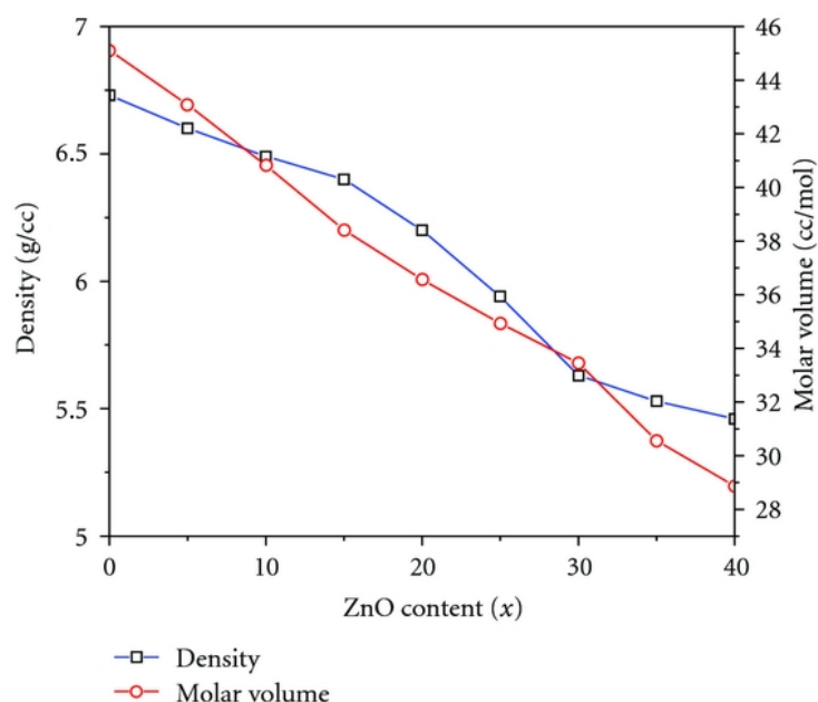
FIGURE 2: Density ( \rho ) and molar quantity ( V_m ) compositional reliance for 40SiO_2 \cdot xZnO \cdot (60 - x)Bi_2O_3 lenses.[27]
