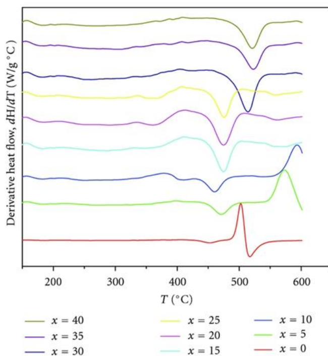
FIGURE 3: Calorimetry differential scanning (DSC) curves for the 40SiO_2 \cdot xZnO \cdot (60 - x)Bi_2O_3 crystal scheme.[27]
