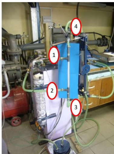
FIGURE 7: An image of the test equipment
