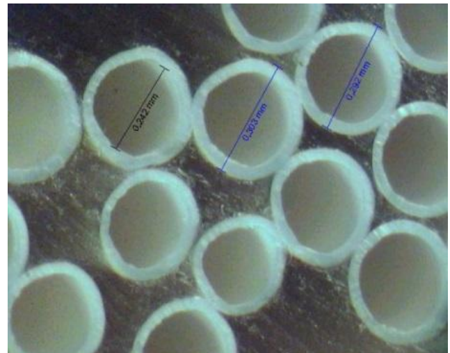
FIGURE 2: A detailed image of the fibres
