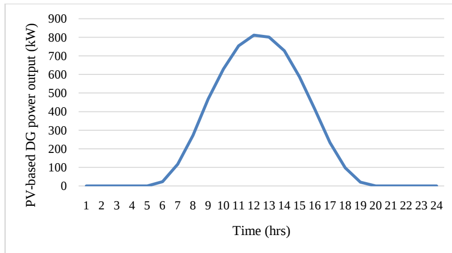
FIGURE 2: Solar power output curve for 24 hrs
