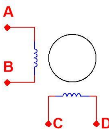
FIGURE 2: 9G Stepper motor configuration [11]
