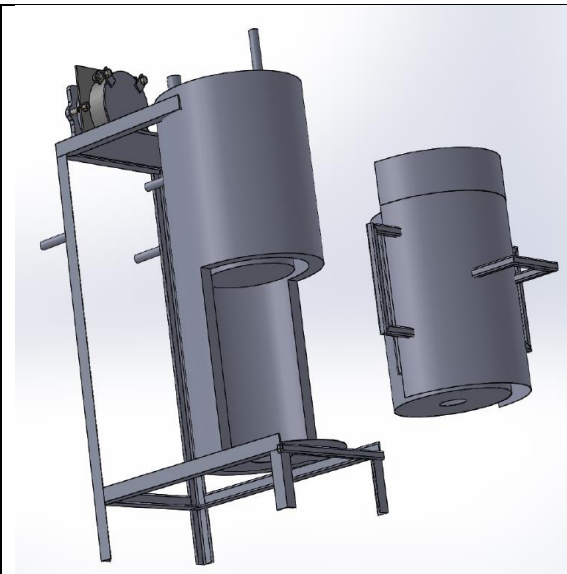
Appendix 5: 3D view of the turbine and the fuel chamber
